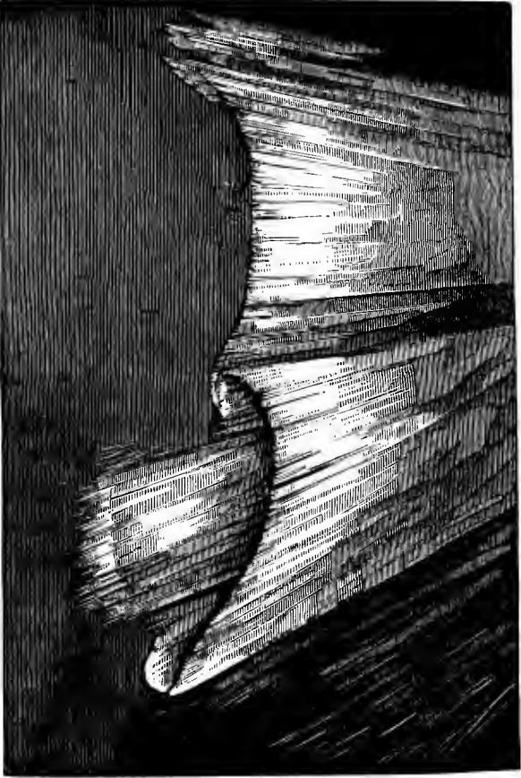
AURORAL CURTAIN SEEN IN SCANDINAVIA
